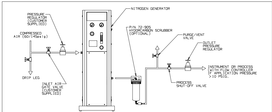
Figure 4 - Recommended Installation
