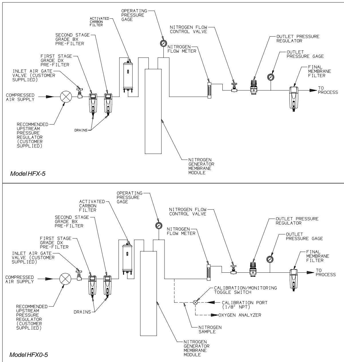
Figure 2 - Flow Schematic
