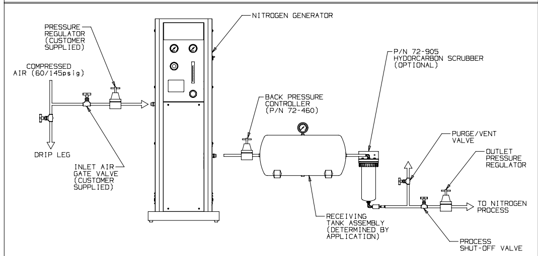
Figure 5 - Receiver Tank Installation
