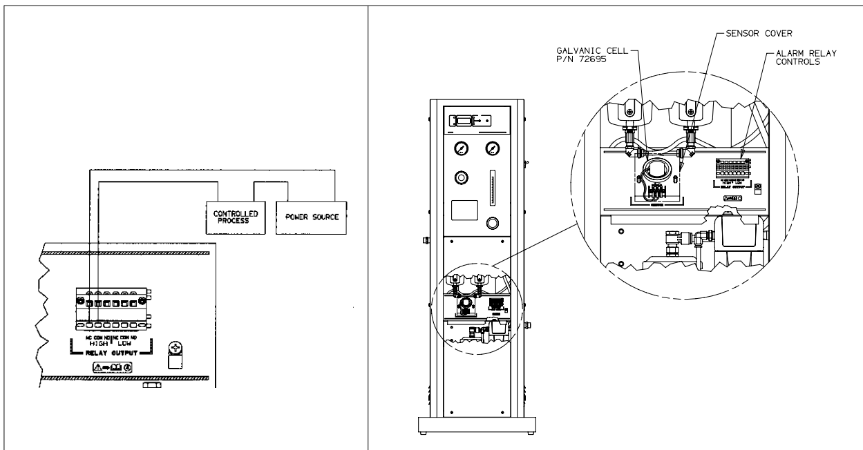
Figure 6 - Sample Wiring Schematic for Alarm Relay Contacts
